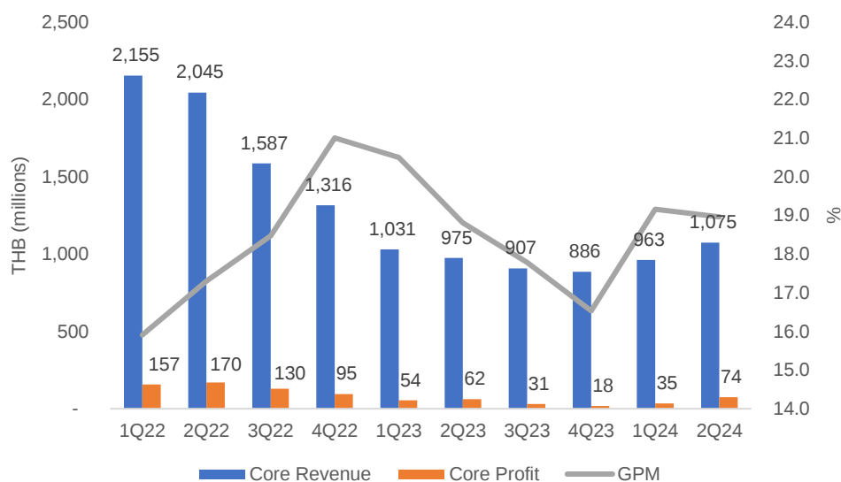
Figure 2: Operating Statistics
